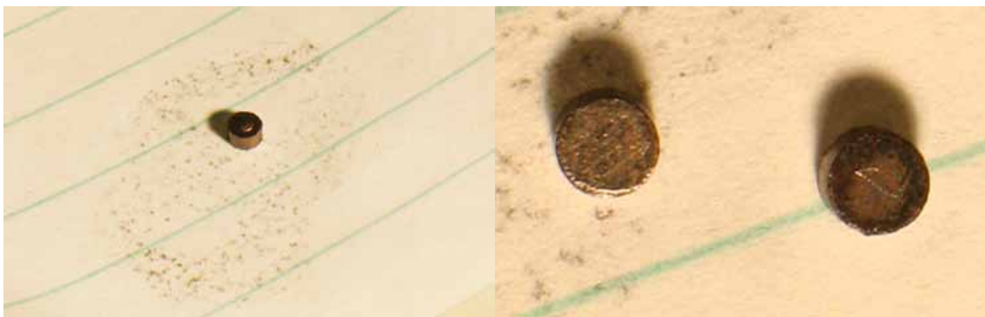
Stock Auto World Motor Brushes and Brush Springs.
