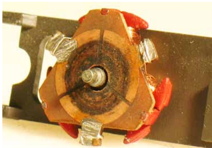
Here is a pancake armature with typical wear and dirt.
