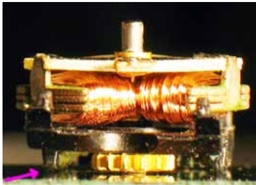
XT Bare Gear Plate Twisted Less than Perfect
