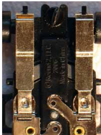
Current Auto World Pick Up Shoe: Wider shoe, long step and more contact area to the track rails.
