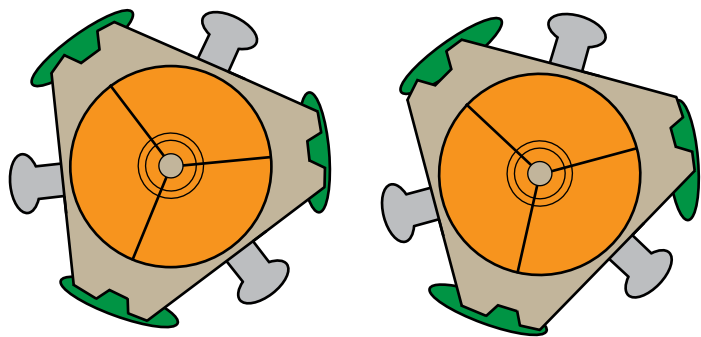
(Left) Zero Degree Stock Armature Timing (Right) Ten Degree Advanced Armature Timing
