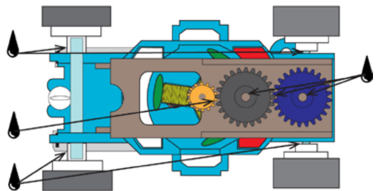
Oiling Chart - Top View
