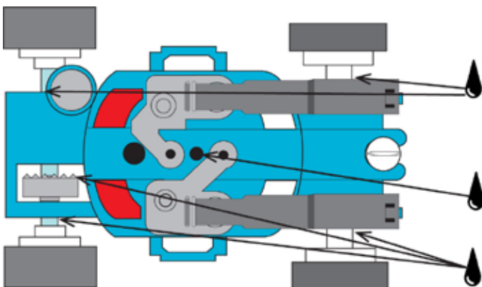
Oiling Chart - Bottom View
